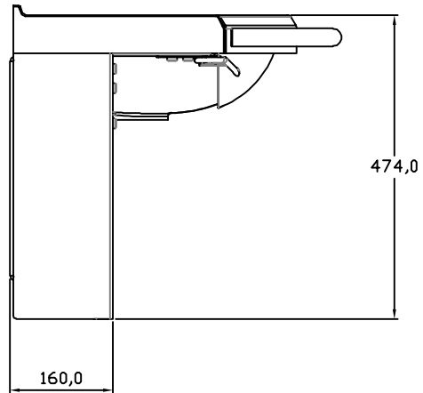
KDR-6401_6514.4_SIDE
