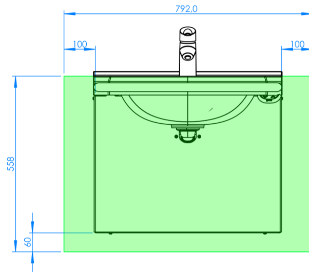
Figure 3. Reinforced area (20 mm plywood with full thread screws)
