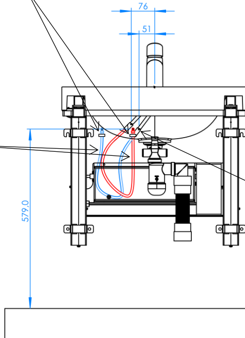
Figure 4. Plumbing view is viewing from the back side of the unit
