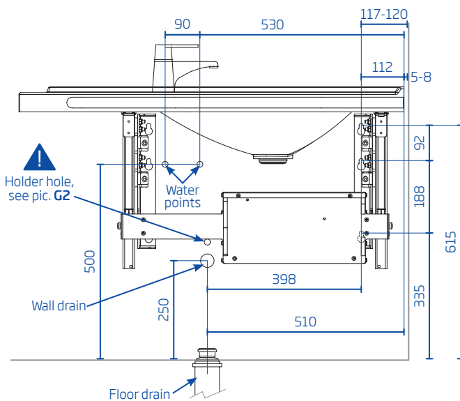
Water and drain places, frame installation measures
